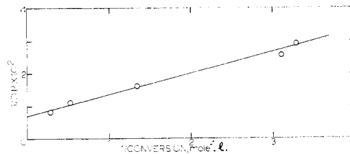
Figure 3. Reciprocal degree of polymerization vs. reciprocal conversion.
